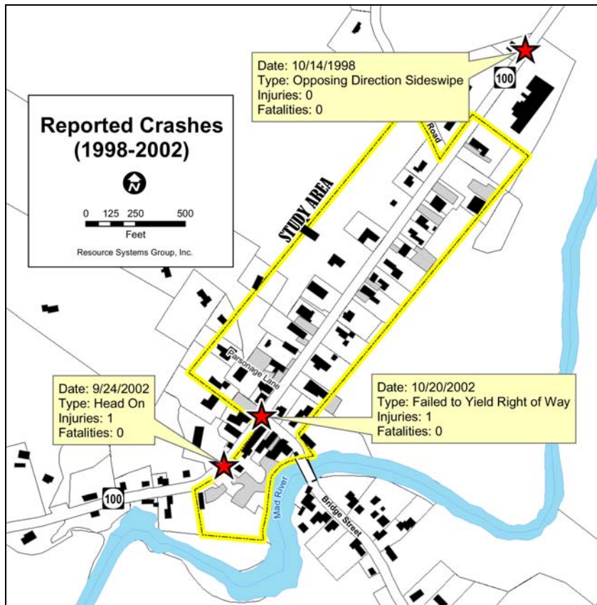
Figure 11: Reported Crashes (1998-2002)
